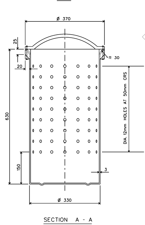
ALUM. ALLOY STRAINER BUCKET
