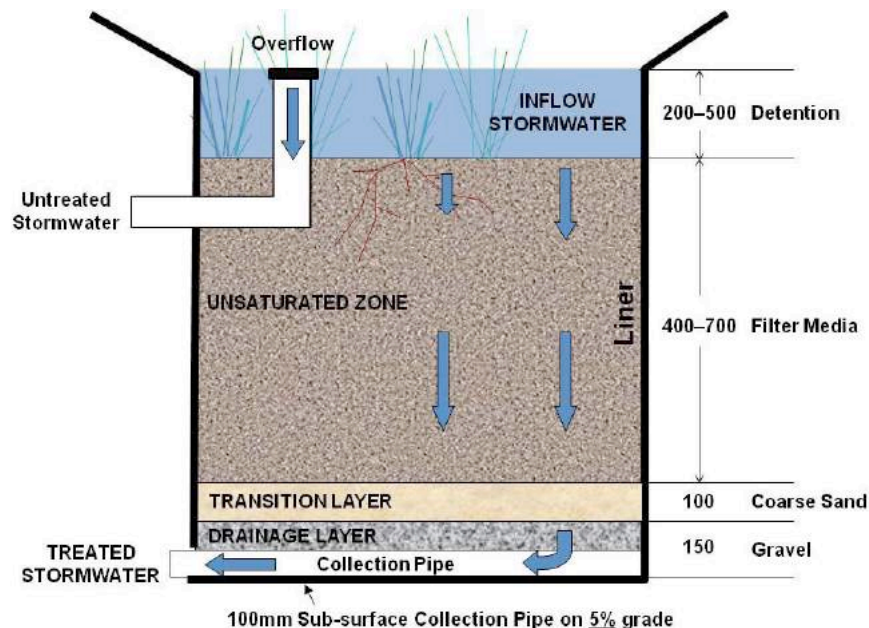
Figure 7.2 Lined standard bioretention system [source: FAWB, 2009]
