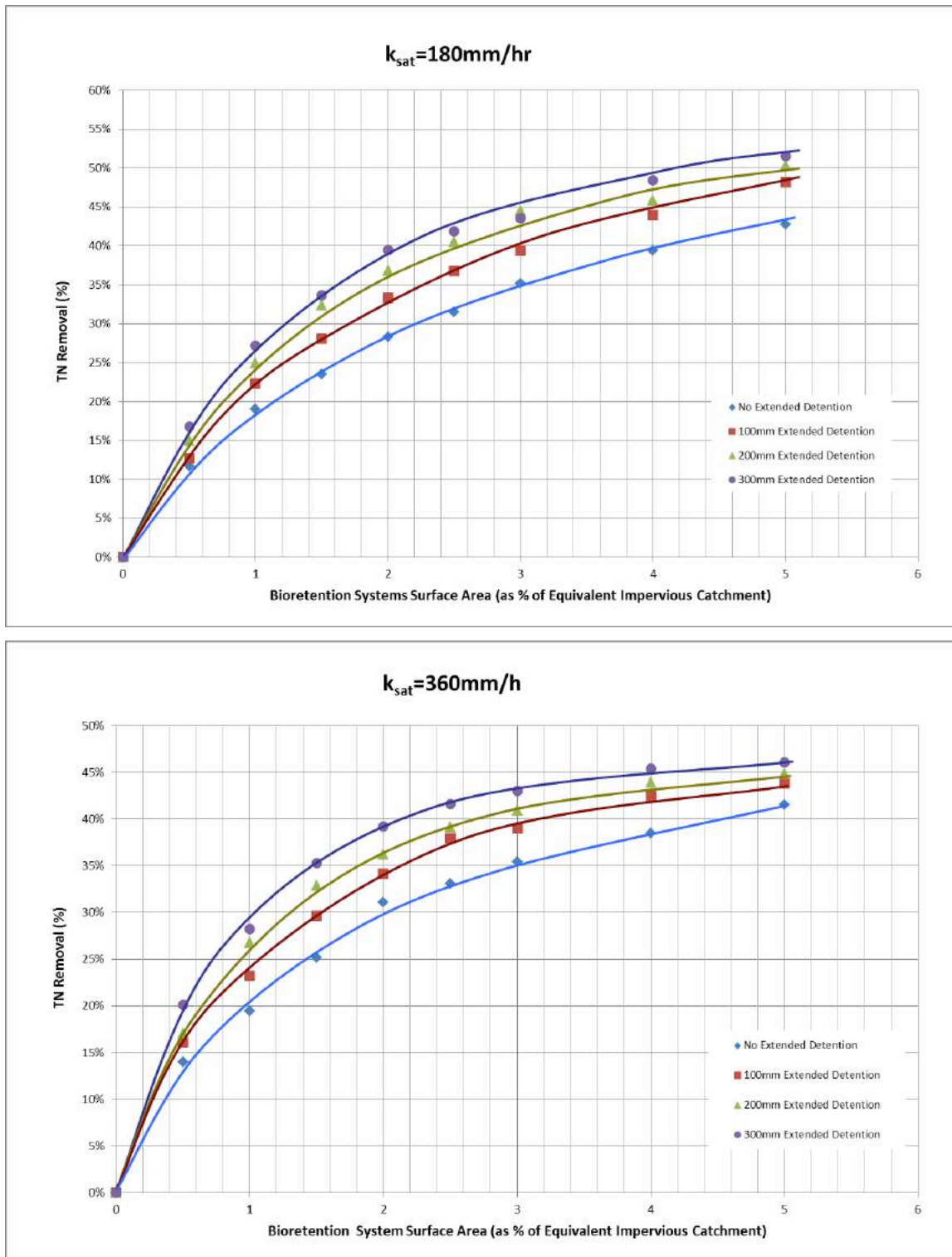
Figure 7.10 Bioretention system TN removal performance (Reference: Station 43)
