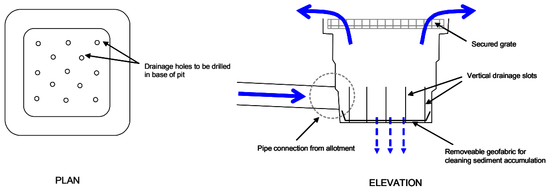
Figure 5.13 Example of Surcharge Pit for Discharging Concentrated Runoff into a Swale
