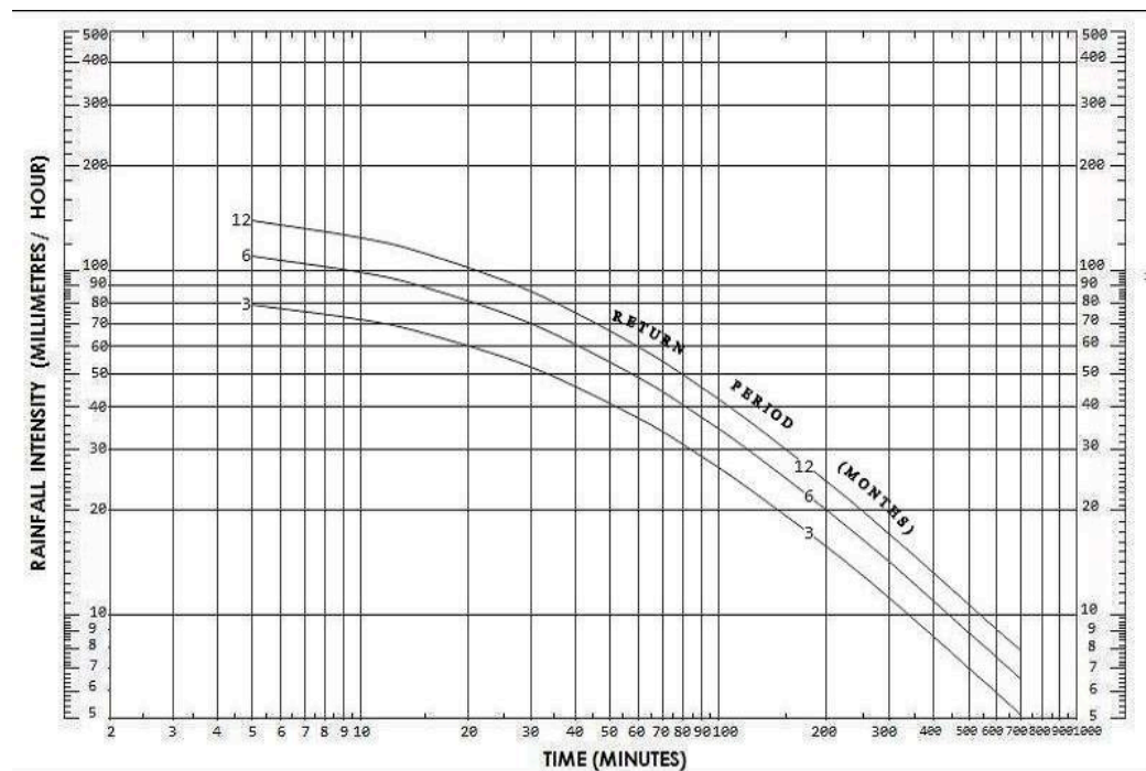
Figure 7.12 IDF Curves for 3-month, 6-month, & 12-month ARI storms
