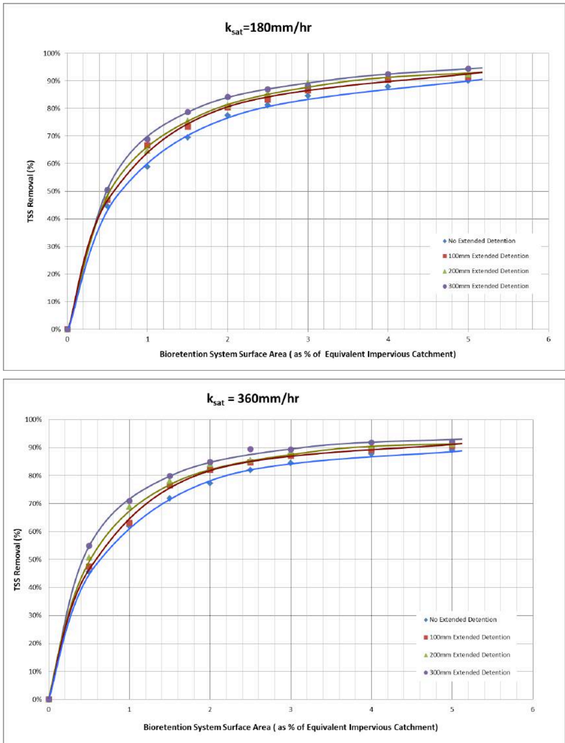
Figure 7.8 Bioretention system TSS removal performance (Reference: Station 43)
