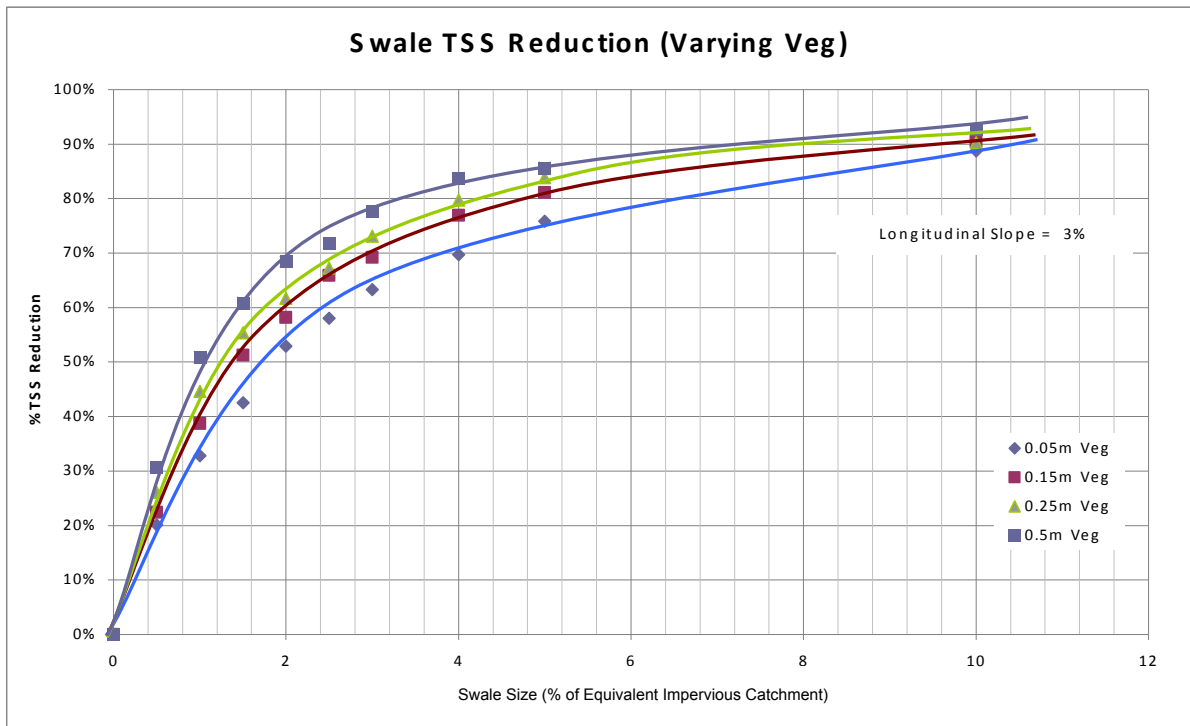
Figure 5.6 Swale TSS Removal Performance
