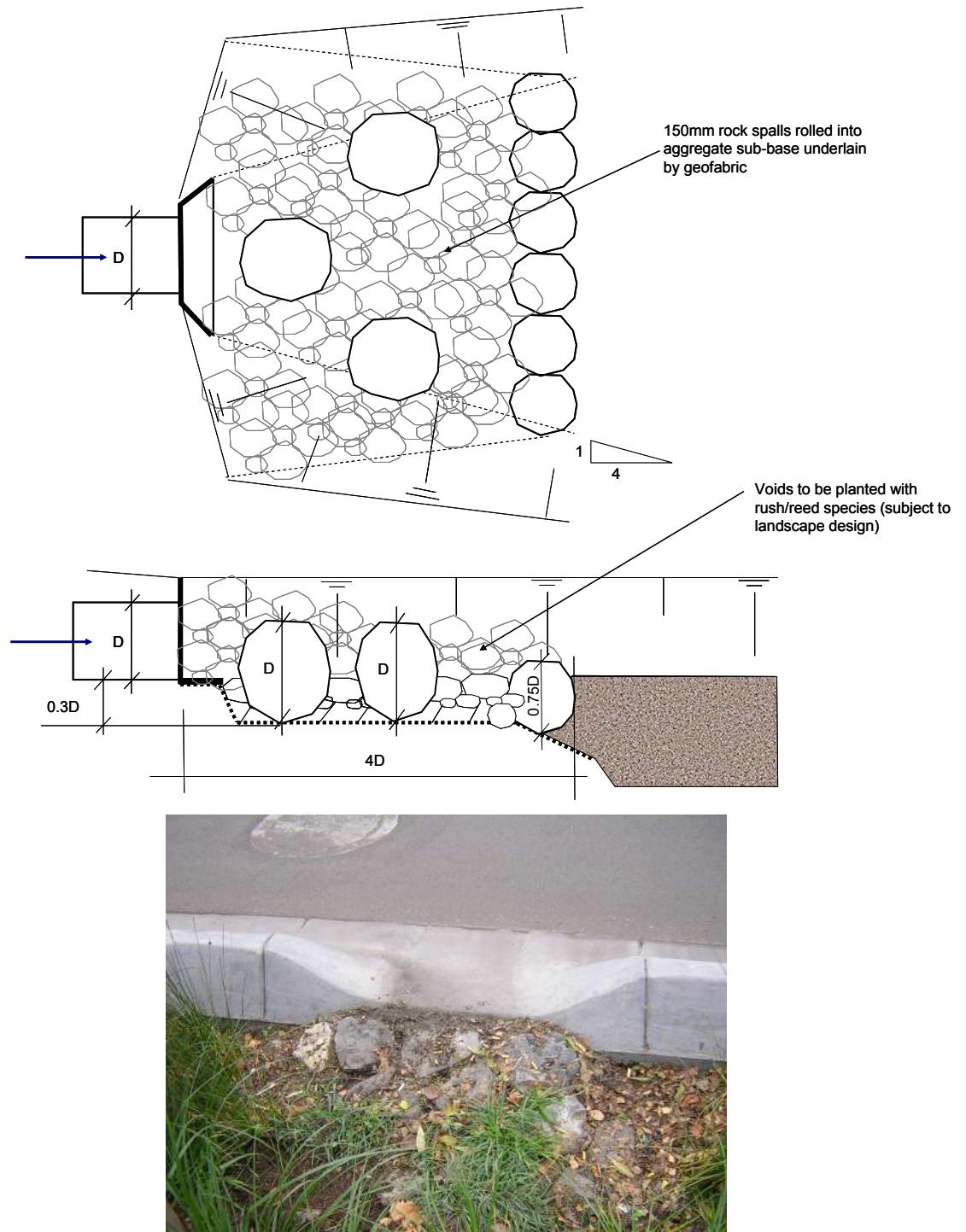
Figure 7.11 Typical Inlet Scour Protection Detail for Bioretention Basins Receiving Piped Flows
