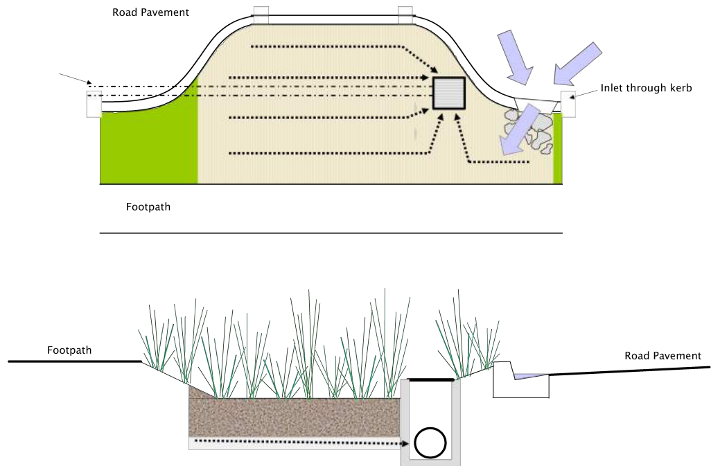
Figure 7.14 Layout of proposed bioretention system
