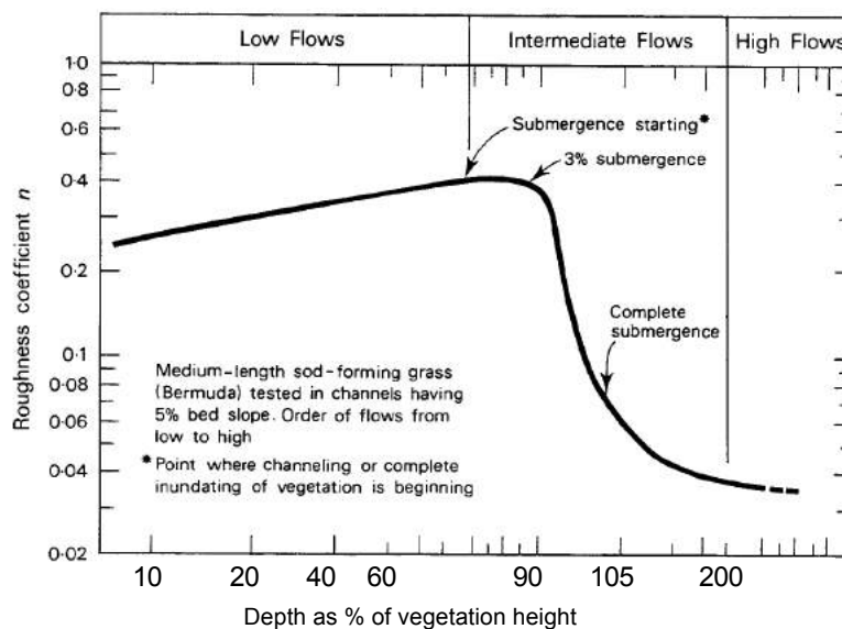
Figure 6.7 Impact of Flow Depth on Hydraulic Roughness (adapted from Barling and Moore (1993))
