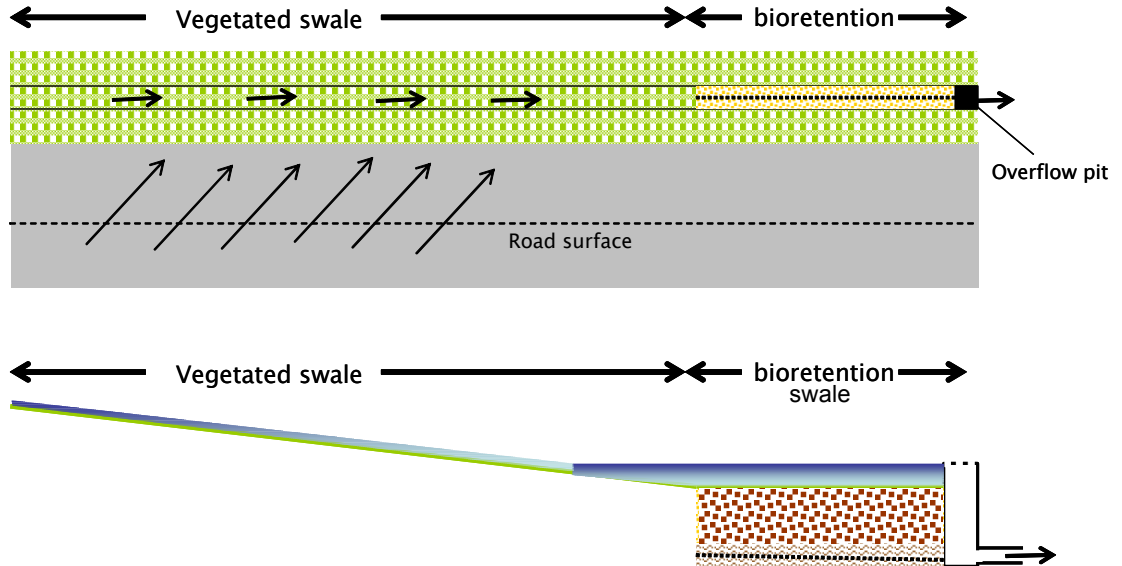
Figure 6.2 Bioretention Swale used downstream of vegetated swale
