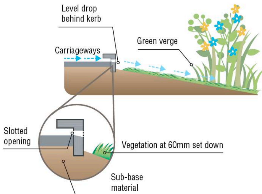
Figure 6.8 Slotted Kerbs with level drop or set-down allow Sediments to Flow into Vegetated Area
