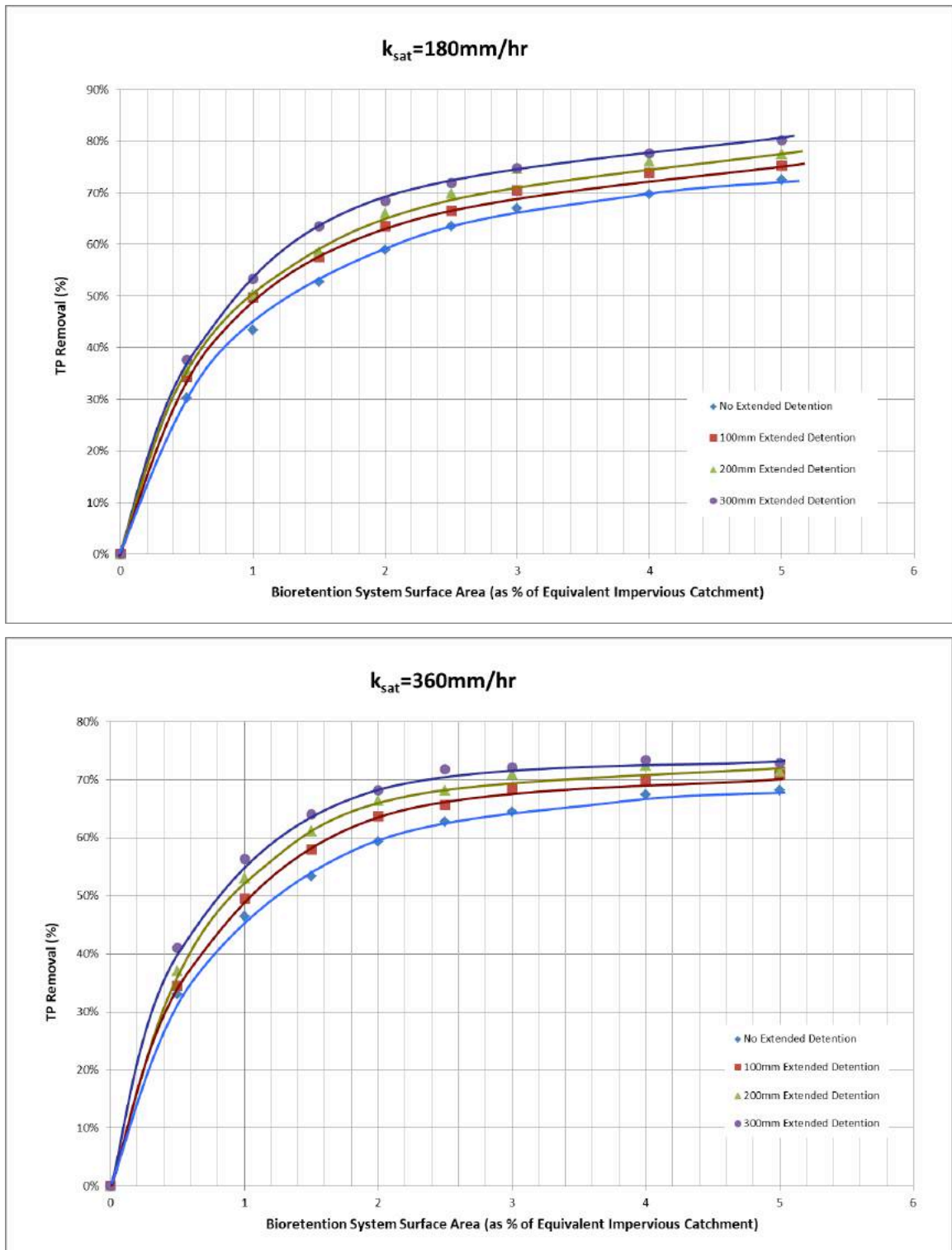
Figure 7.9 Bioretention system TP removal performance (Reference: Station 43)
