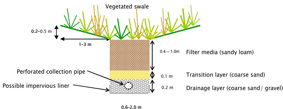
Figure 6.3 Typical Section of a Bioretention Swale
