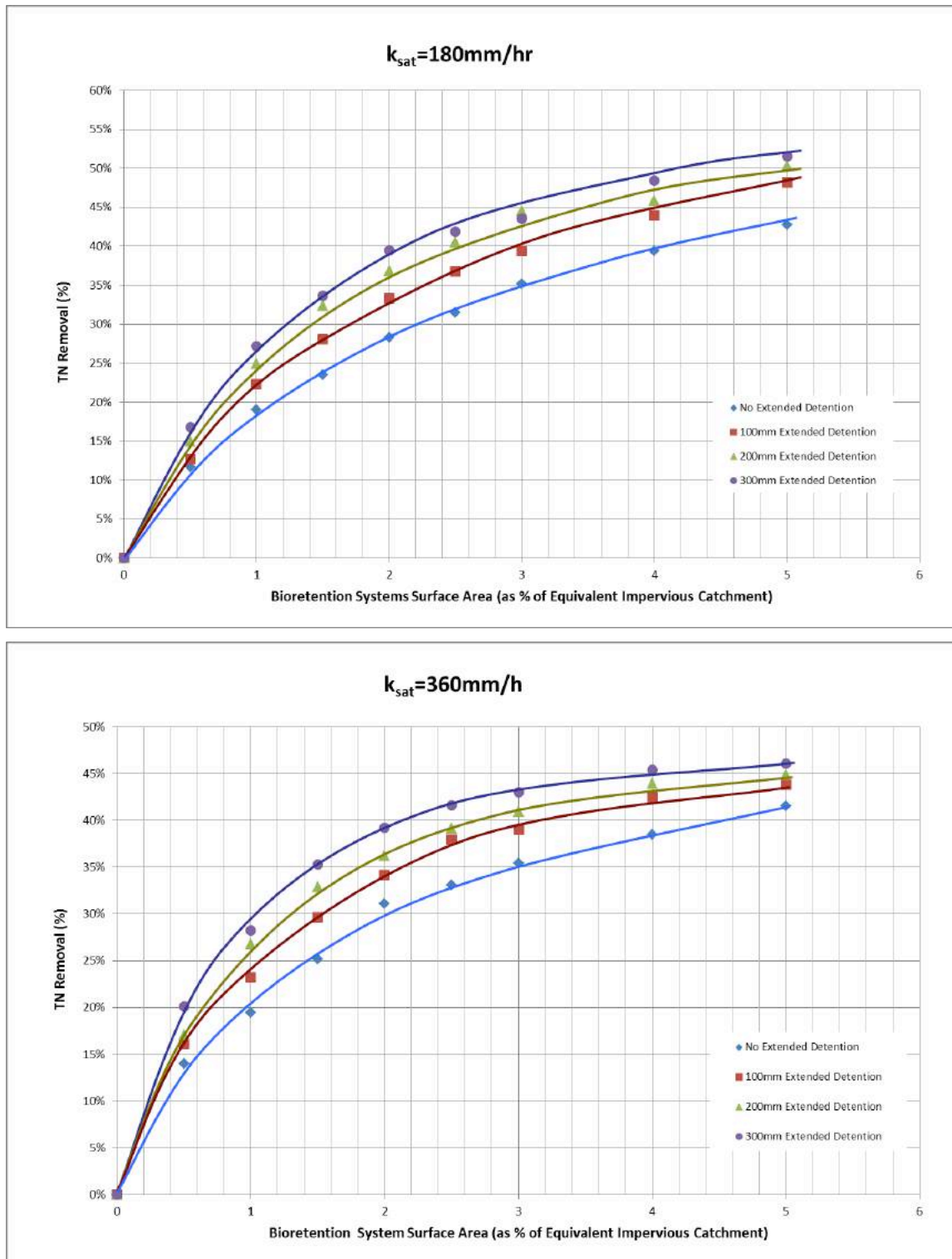
Figure 6.6 Bioretention system TN removal performance (Reference: Station 43)
