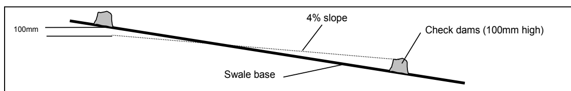
Figure 5.2: Location of Check Dams in Swales
