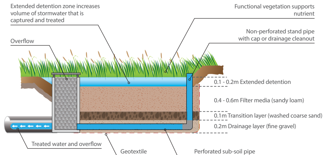
Figure 7.7 Typical cross section of a bioretention basin
