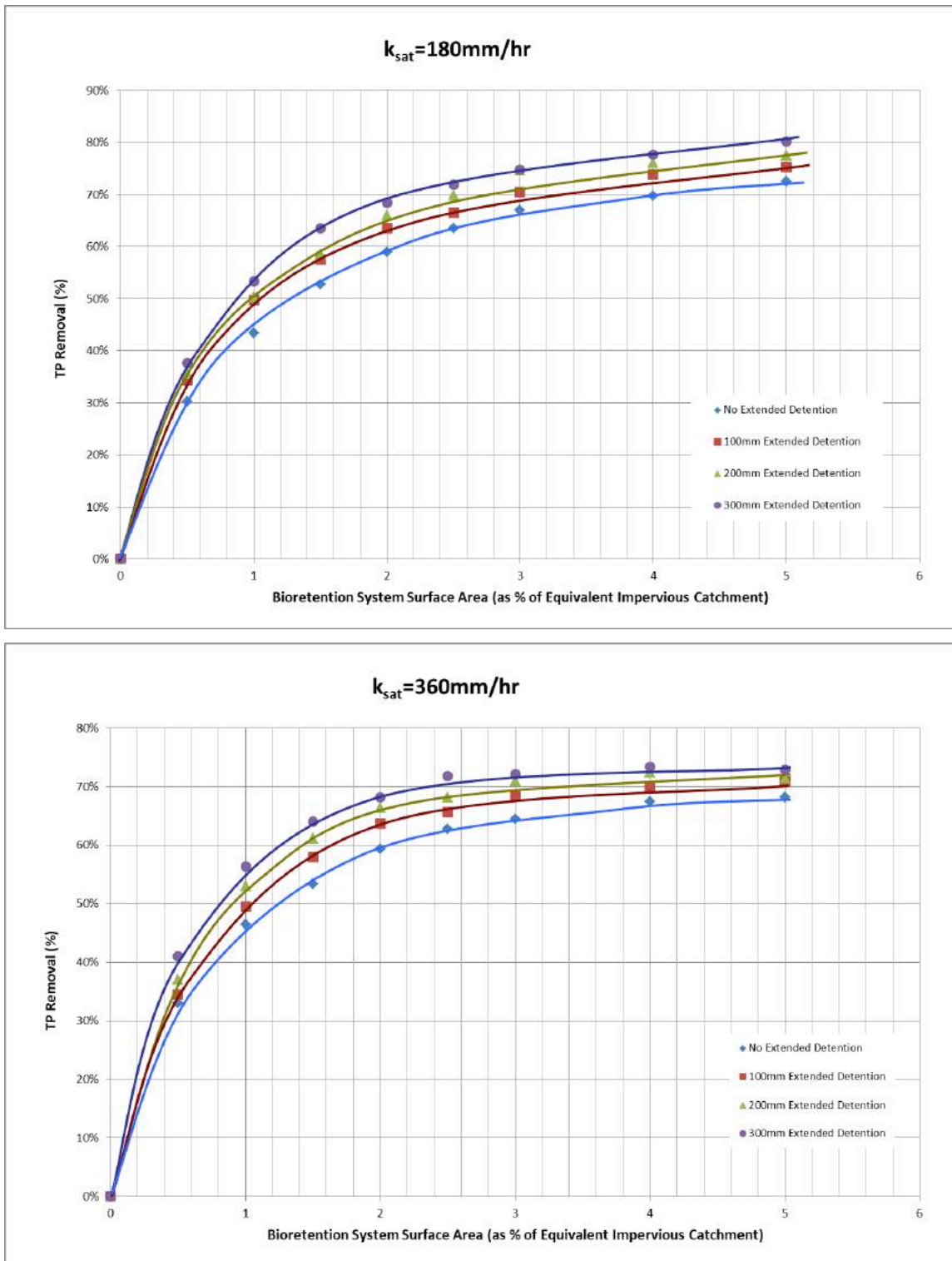
Figure 6.5 Bioretention system TP removal performance (Reference: Station 43)
