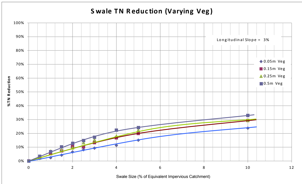
Figure 5.8 Swale TN Removal Performance
