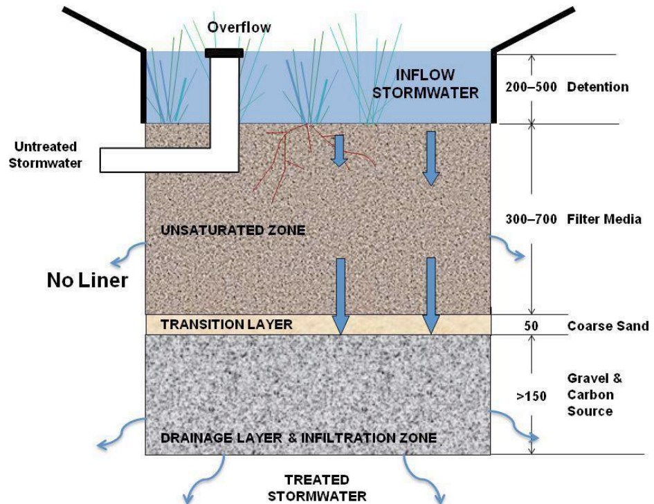
Figure 7.6 A hybrid bioretention and infiltration system [source: FAWB, 2009]
