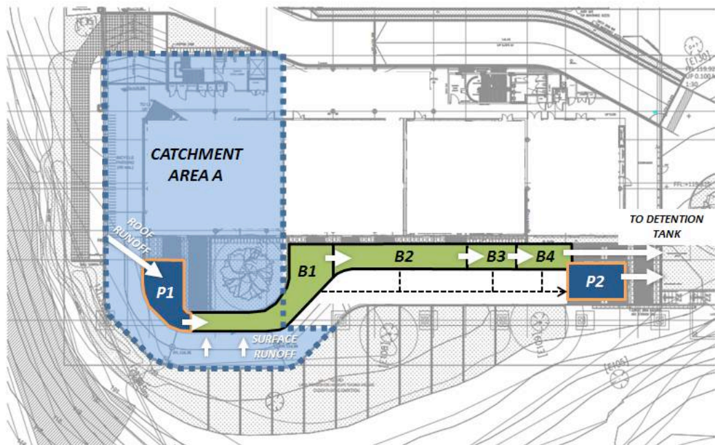
Figure 7.16 Site Plan
