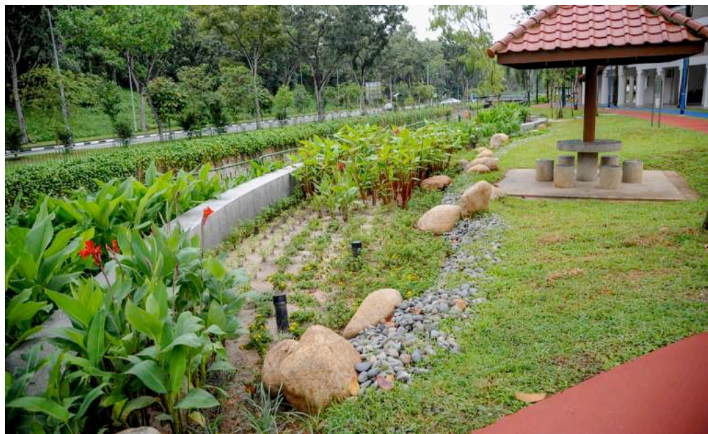
Figure 7.1 Examples of bioretention basin integrated into a local residential area
