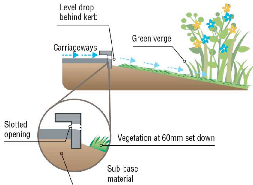
Figure 5.11 Slotted kerb with set-down to allow sediment to flow into the vegetated area
