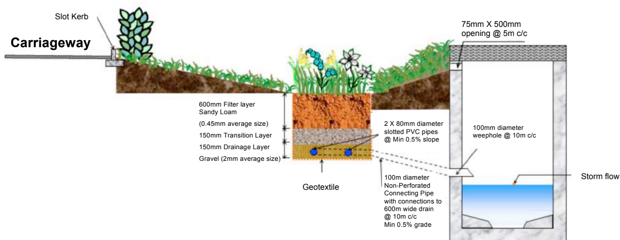
Figure 6.1 A typical Bioretention swale
