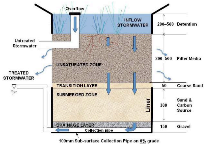
Figure 7.5 Unlined bioretention system with submerged zone [source: FAWB, 2009]
