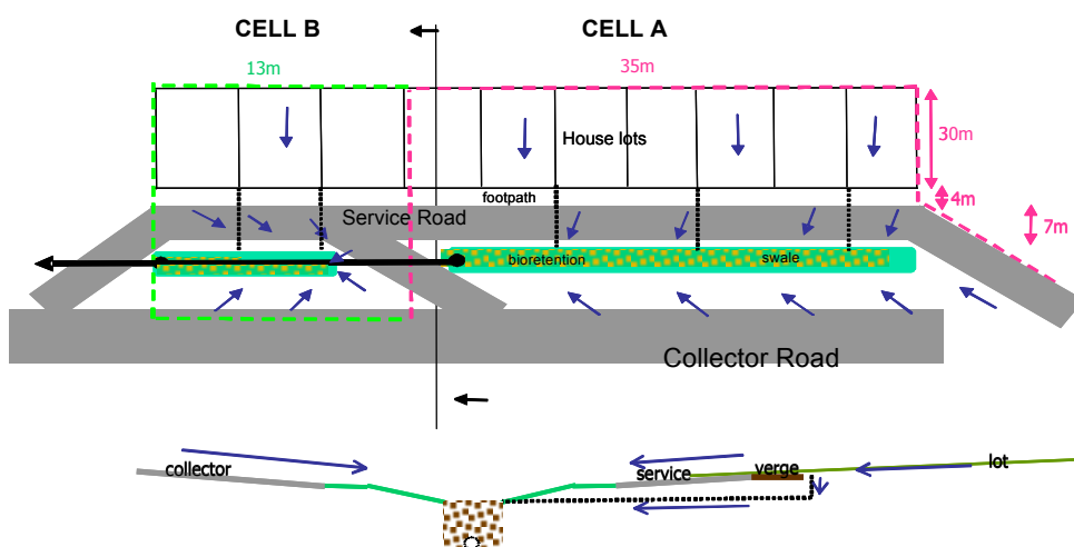
Figure 6.12 Catchment area layout and section for worked example
