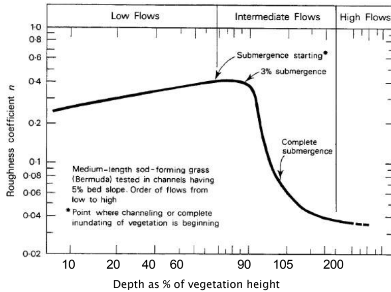
Figure 5.9 Impact of Flow Depth on Hydraulic Roughness (adapted from Barling & Moore (1993))
