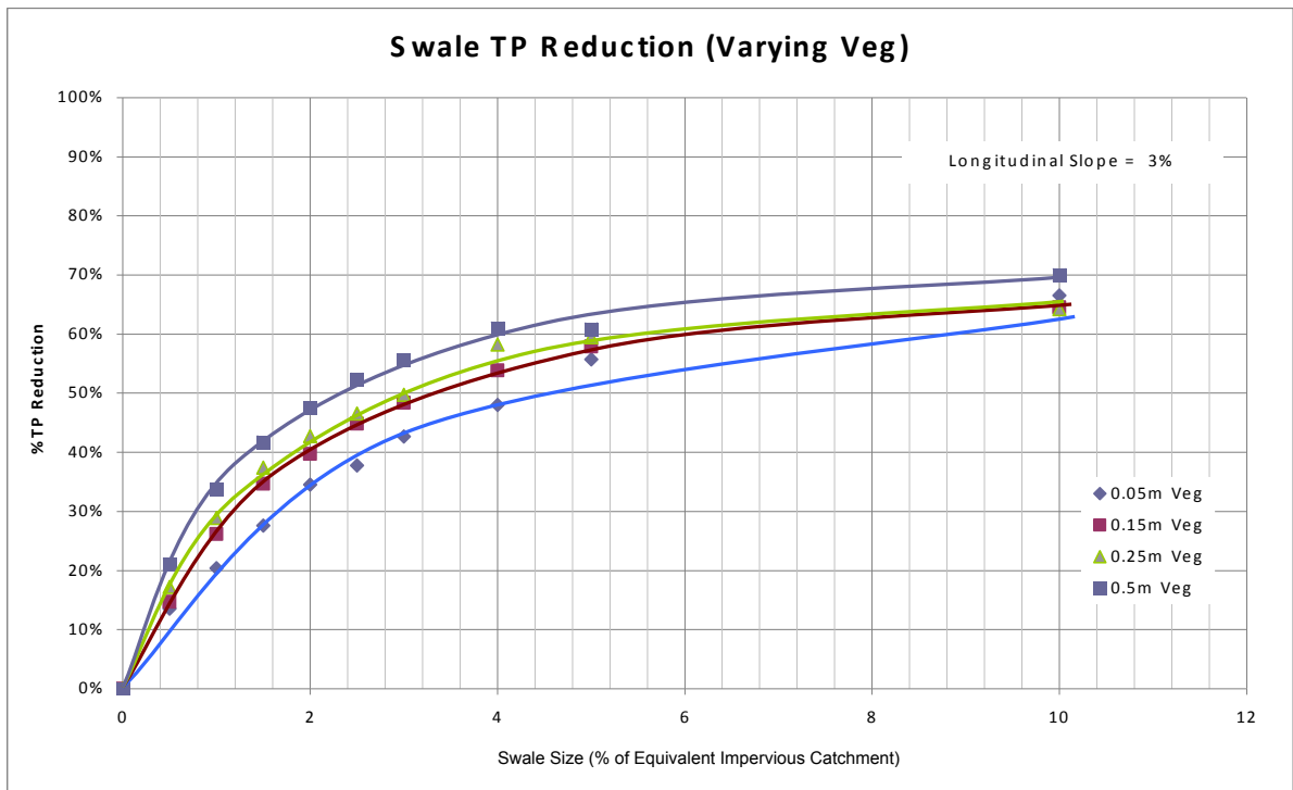
Figure 5.7 Swale TP Removal Performance
