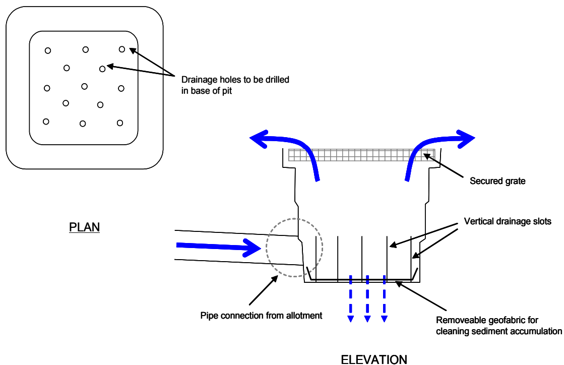
Figure 6.11 Example of Surcharge Pit for Discharging Allotment Runoff into a Swale
