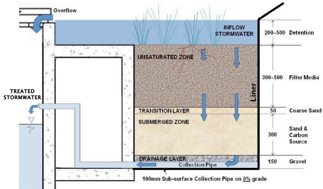
Figure 7.3 Lined bioretention system with submerged zone comprised of gravels and hardwood chips [modified from: FAWB, 2009]
