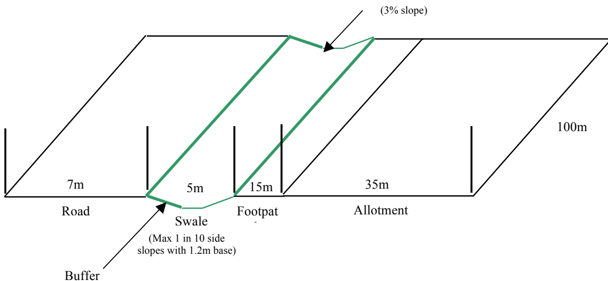
Figure 5.14 Cross section of proposed buffer/swale system
