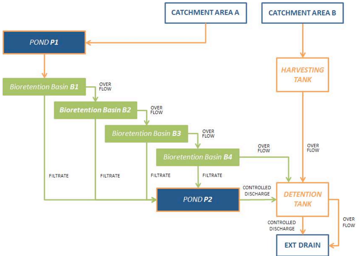
Figure 7.17 Schematic diagram of the bioretention and pond system
