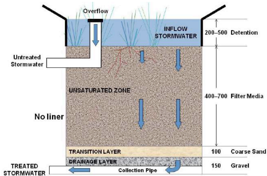
Figure 7.4 Unlined standard bioretention system [source: FAWB, 2009]
