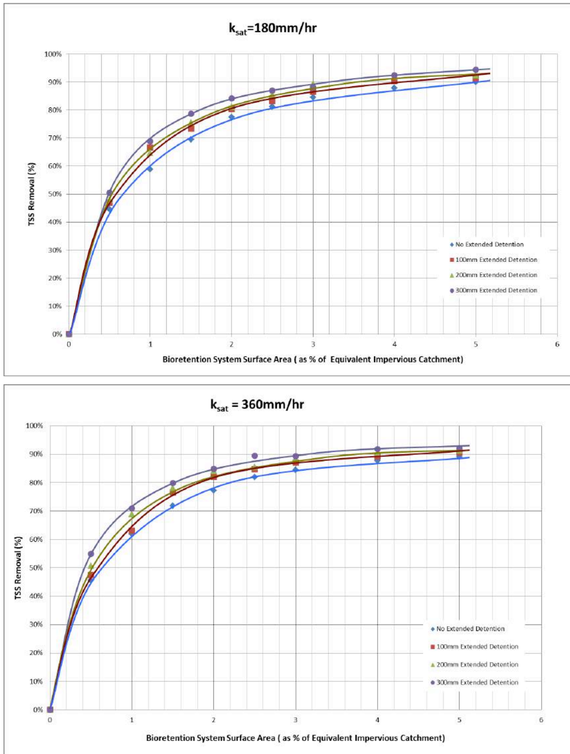
Figure 6.4 Bioretention system TSS removal performance (Reference: Station 43)
